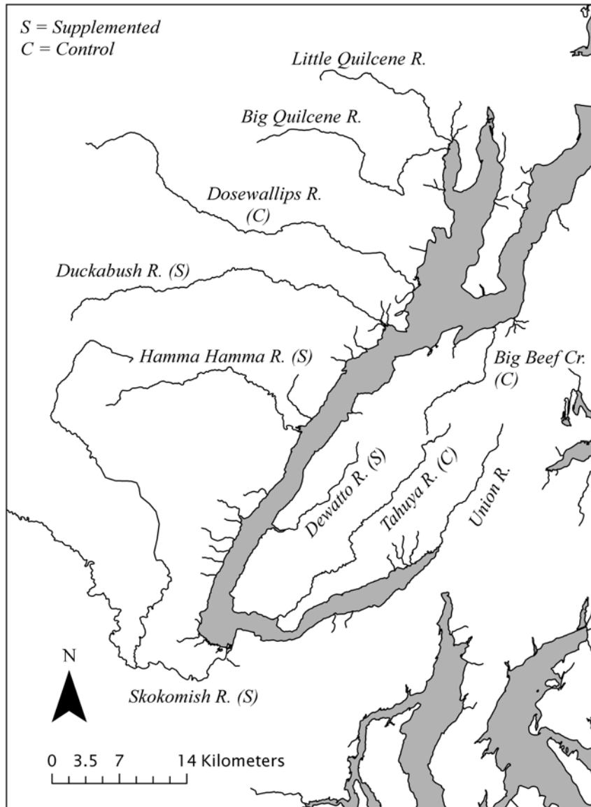
Figure 1. Locations of the supplemented (S) and control (C) streams in Hood Canal.
